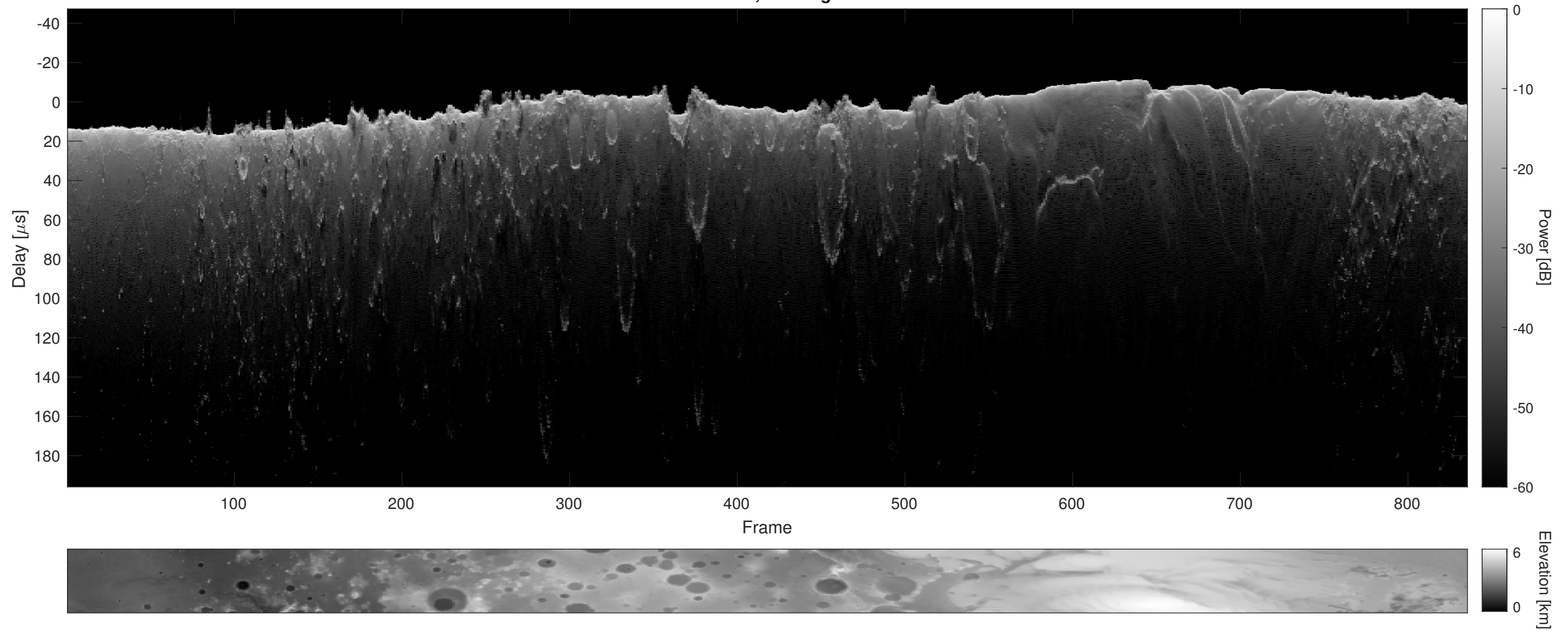
Orbit 6721, Cluttergram
