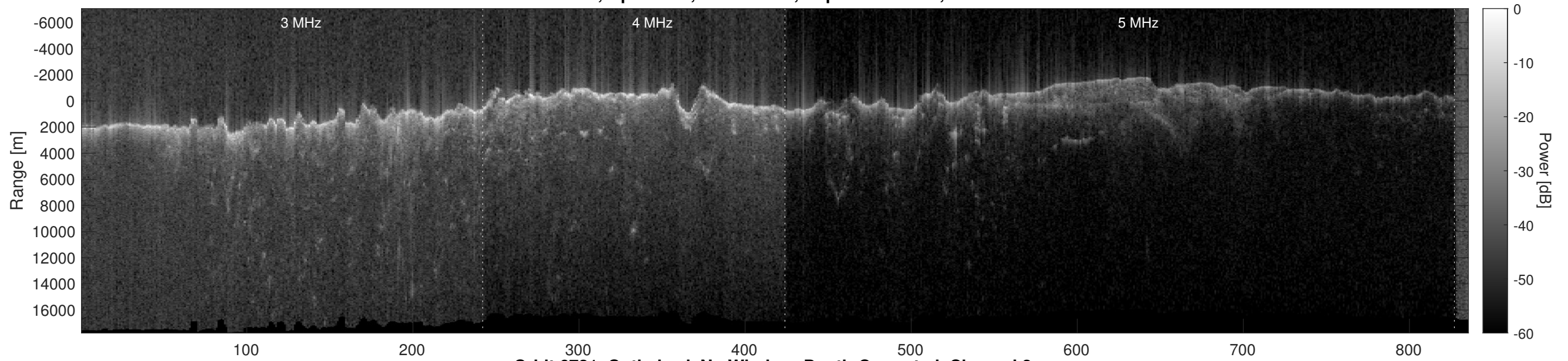
Orbit 6721, Optimized, No Window, Depth-Corrected, Channel 2
