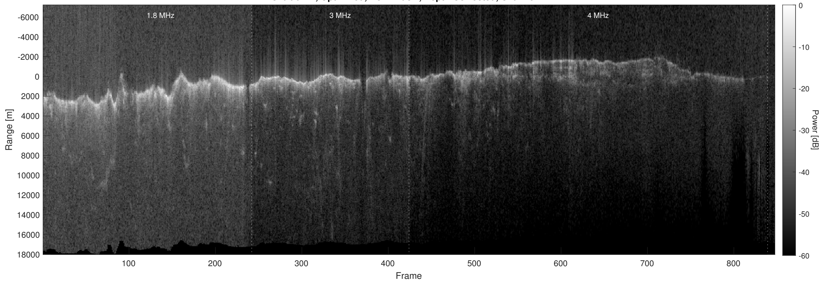
Orbit 6724, Optimized, No Window, Depth-Corrected, Channel 2
