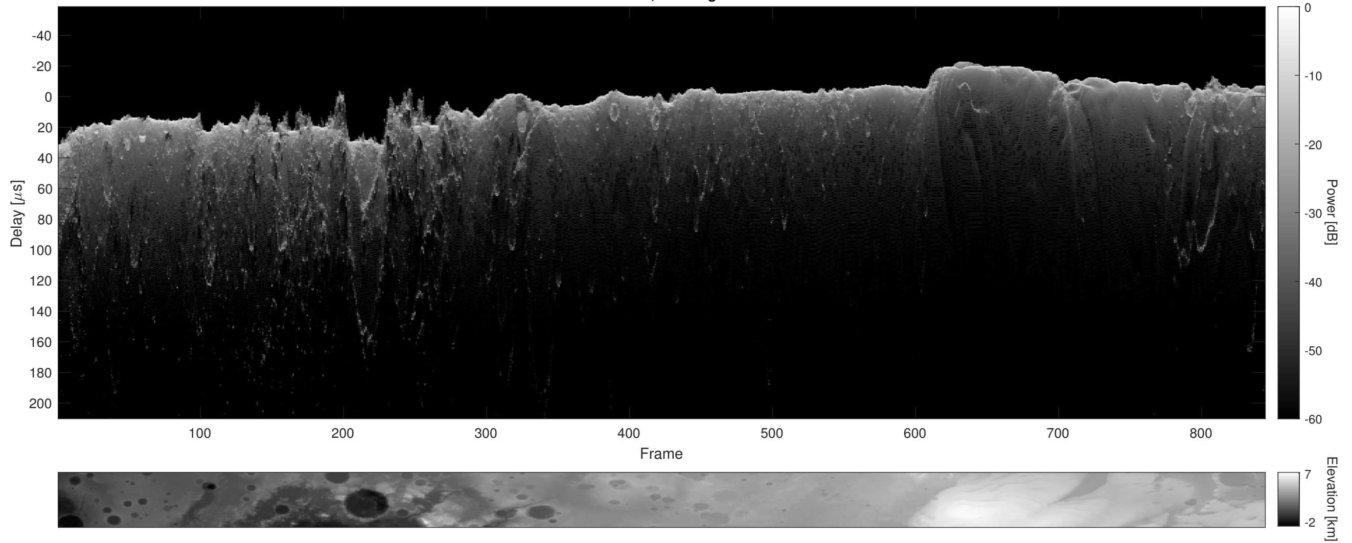
Orbit 6726, Cluttergram
