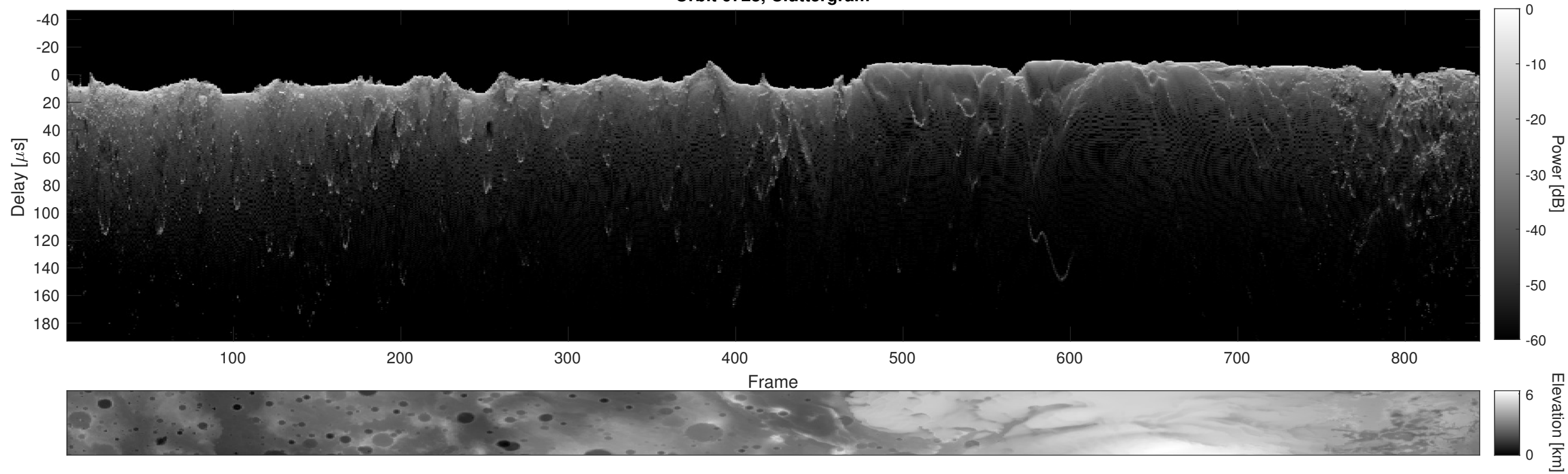
Orbit 6728, Cluttergram
