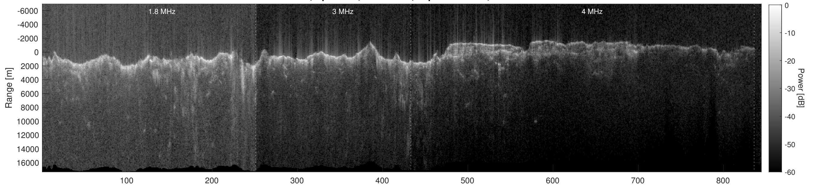
Orbit 6728, Depth-Corrected Cluttergram
