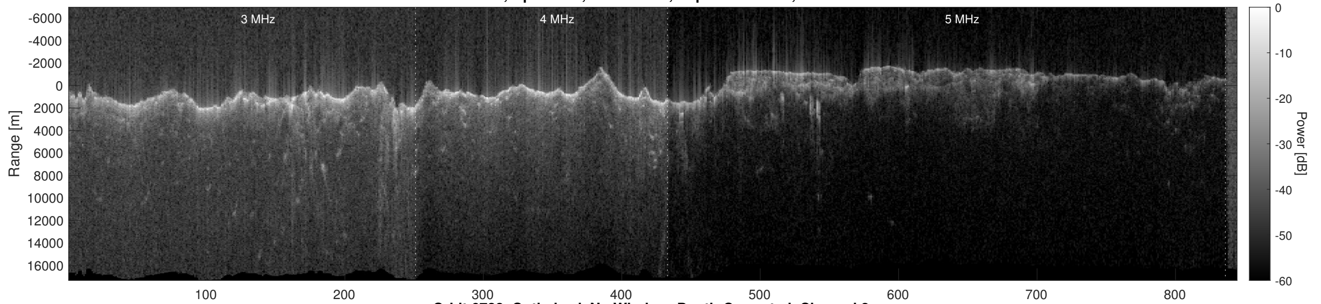
Orbit 6728, Optimized, No Window, Depth-Corrected, Channel 2
