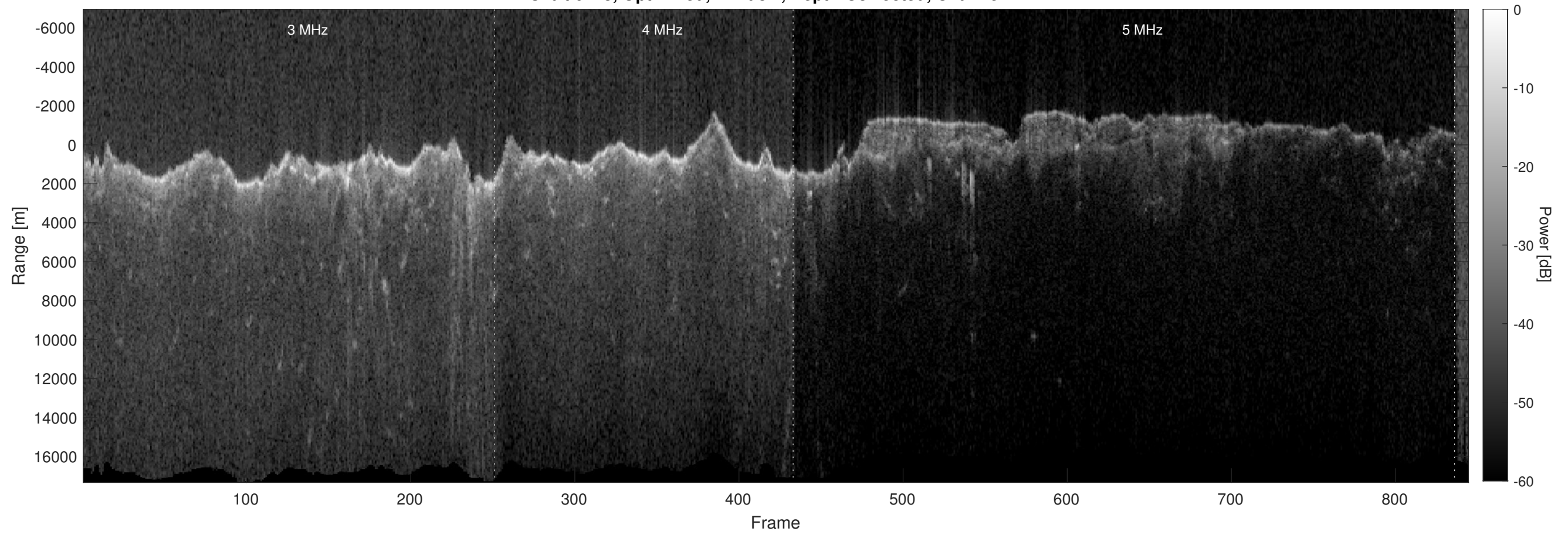
Orbit 6728, Optimized, Window, Depth-Corrected, Channel 2
