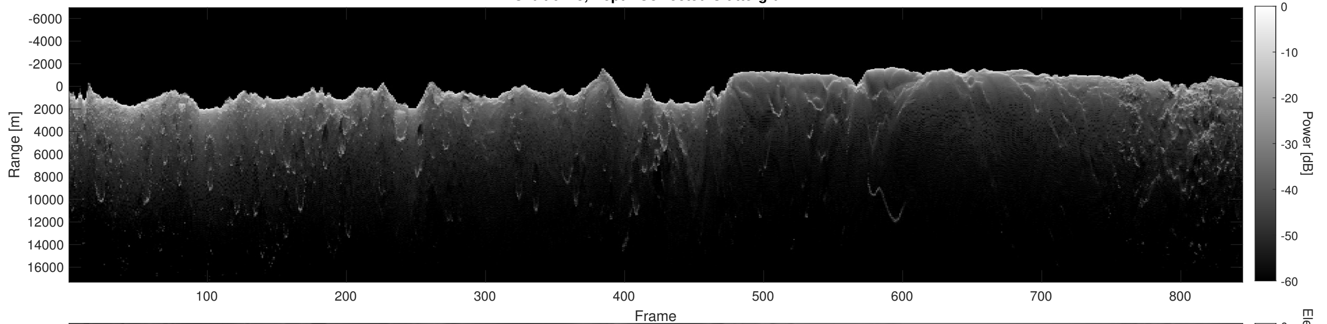
Orbit 6728, Depth-Corrected Cluttergram
