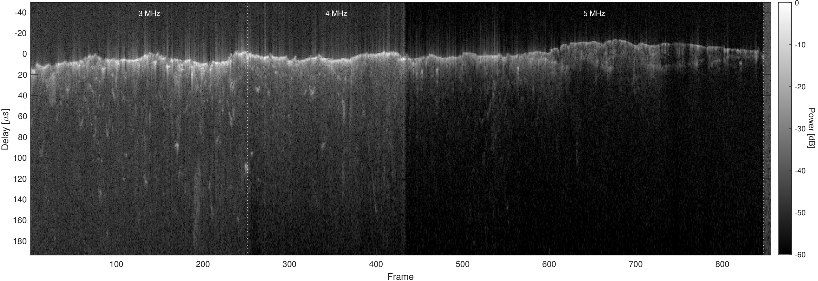
Orbit 6729, Optimized, No Window, Channel 2
