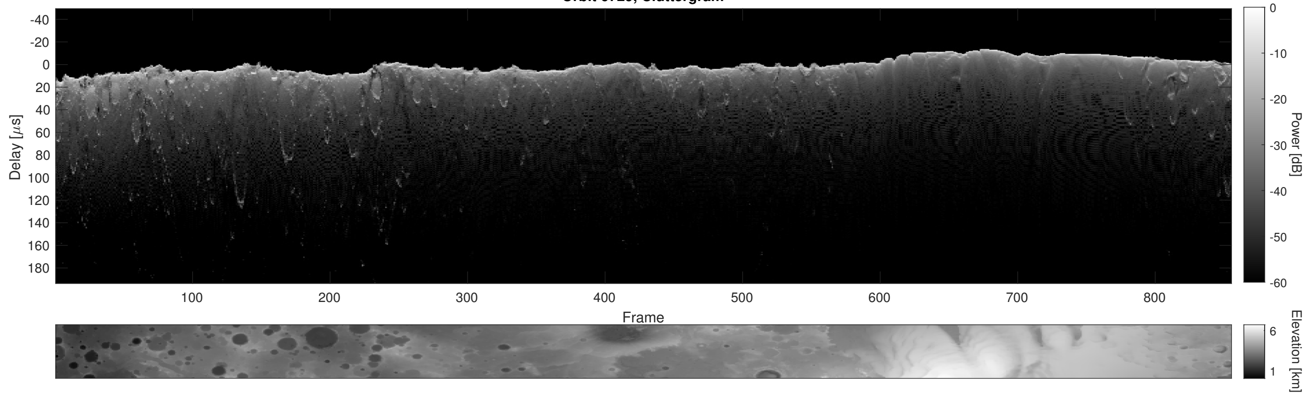
Orbit 6729, Cluttergram
