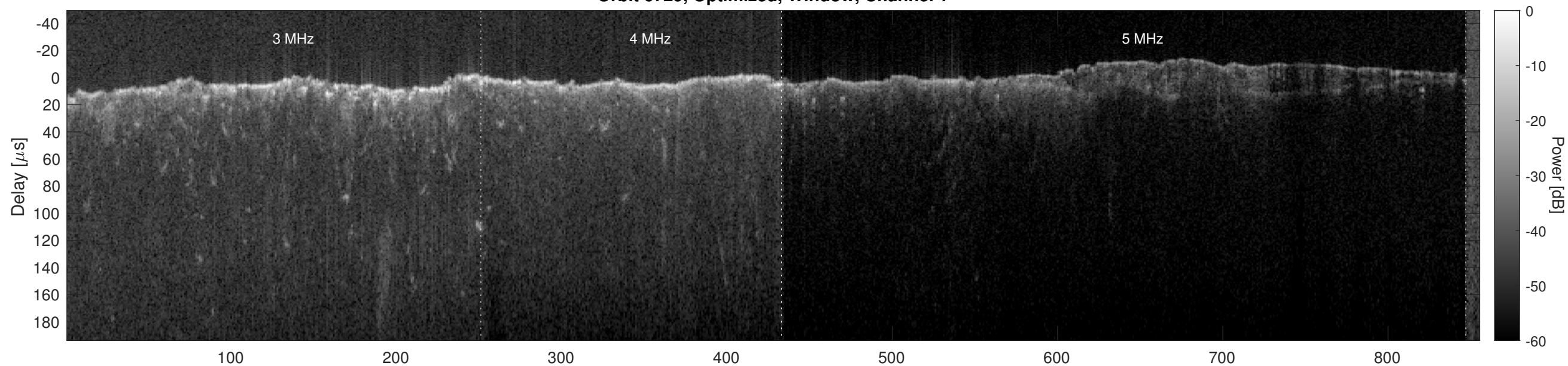
Orbit 6729, Optimized, Window, Channel 2
