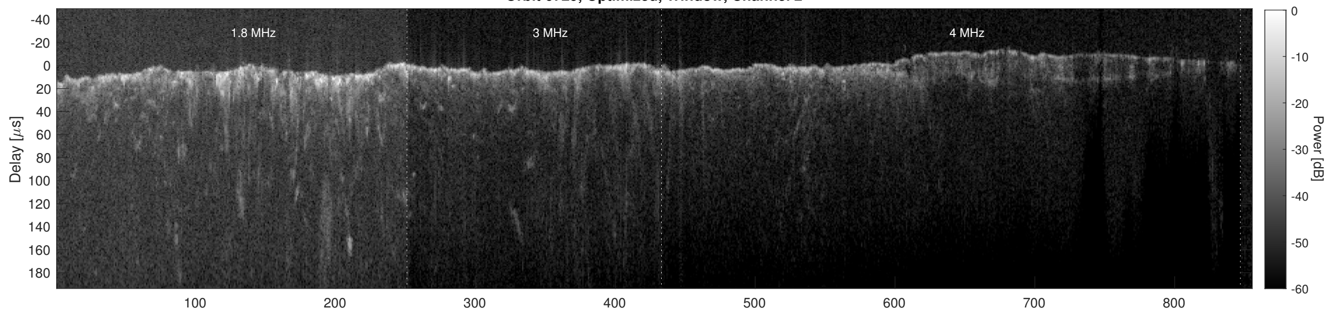
Orbit 6729, Cluttergram
