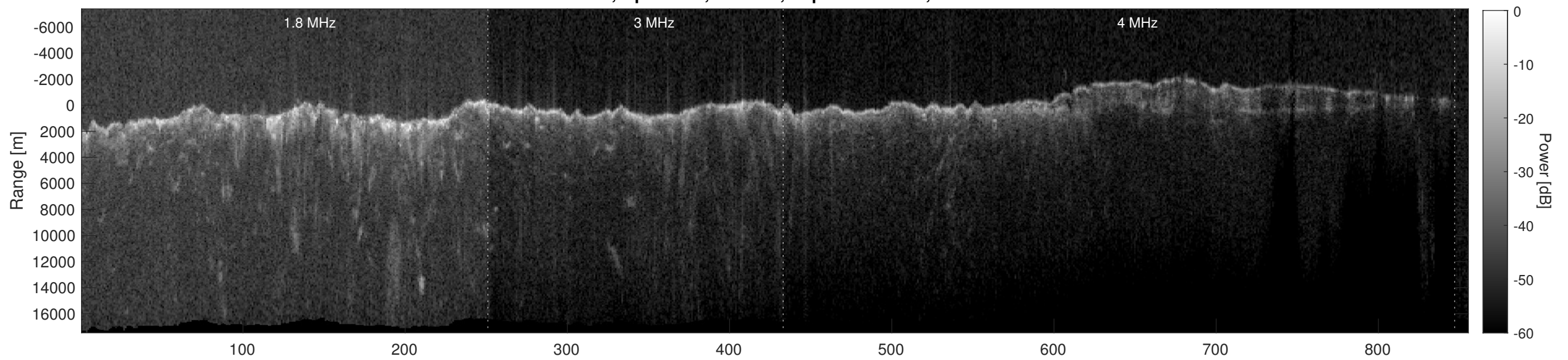
Orbit 6729, Depth-Corrected Cluttergram
