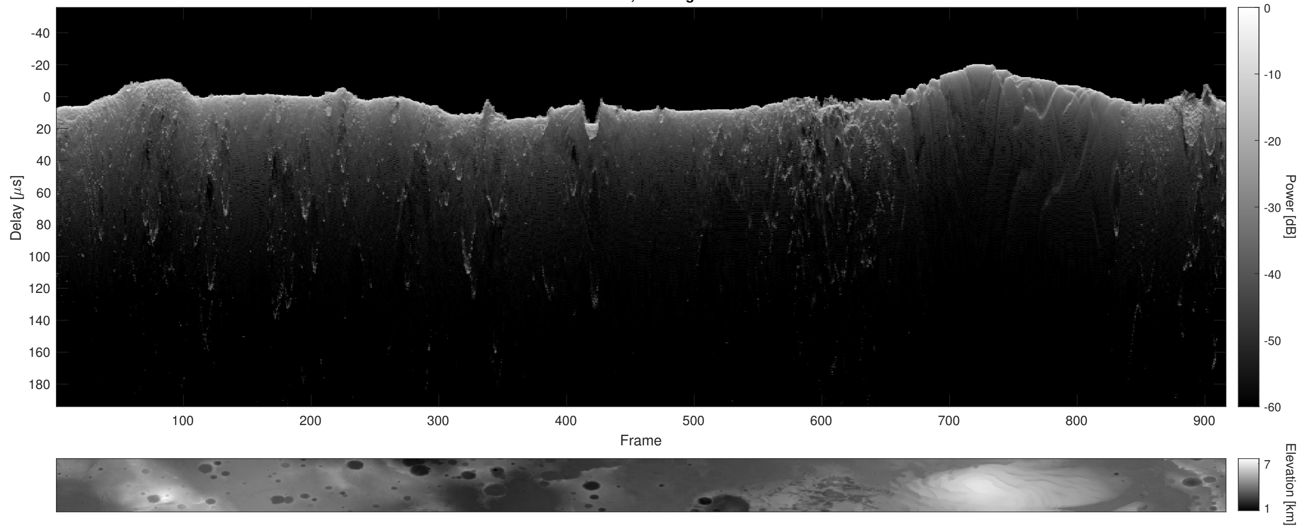
Orbit 6730, Cluttergram
