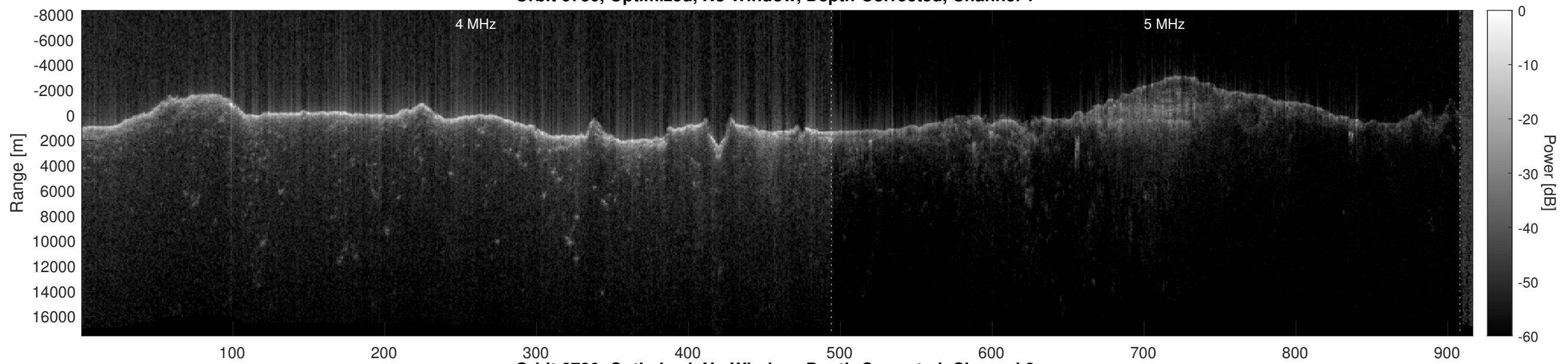
Orbit 6730, Optimized, No Window, Depth-Corrected, Channel 2
