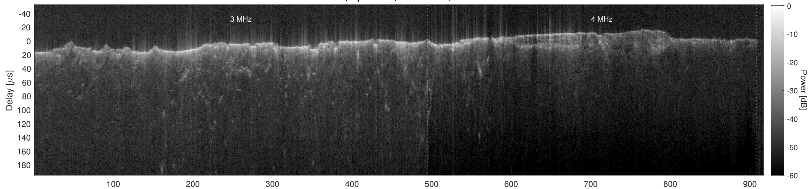
Orbit 6731, Cluttergram
