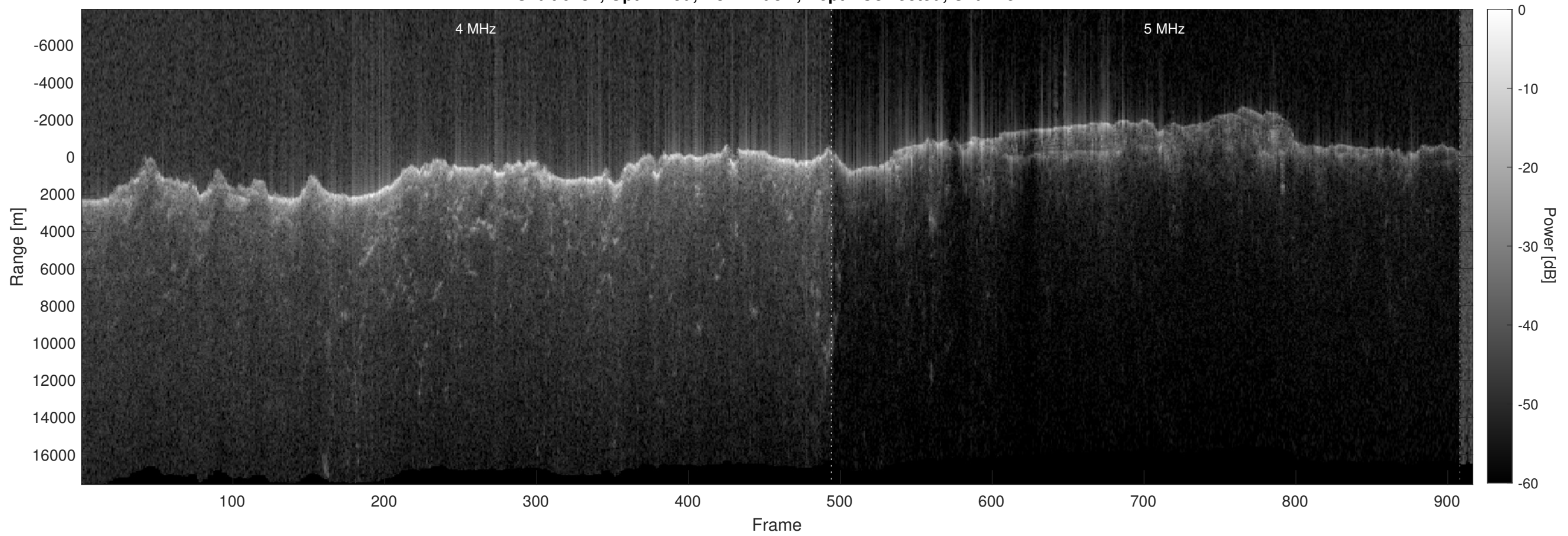
Orbit 6731, Optimized, No Window, Depth-Corrected, Channel 2
