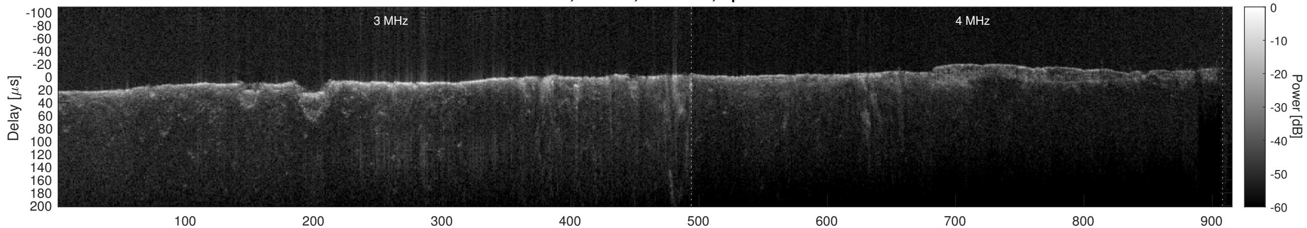
Orbit 6733, Cluttergram
