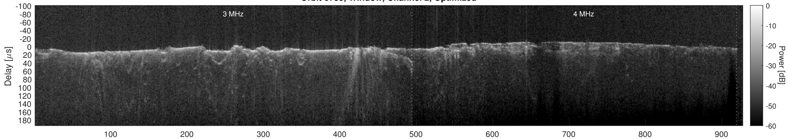
Orbit 6735, Cluttergram
