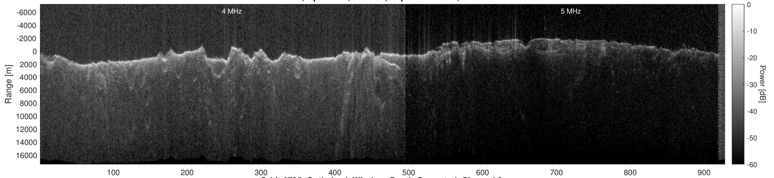
Orbit 6735, Optimized, Window, Depth-Corrected, Channel 2
