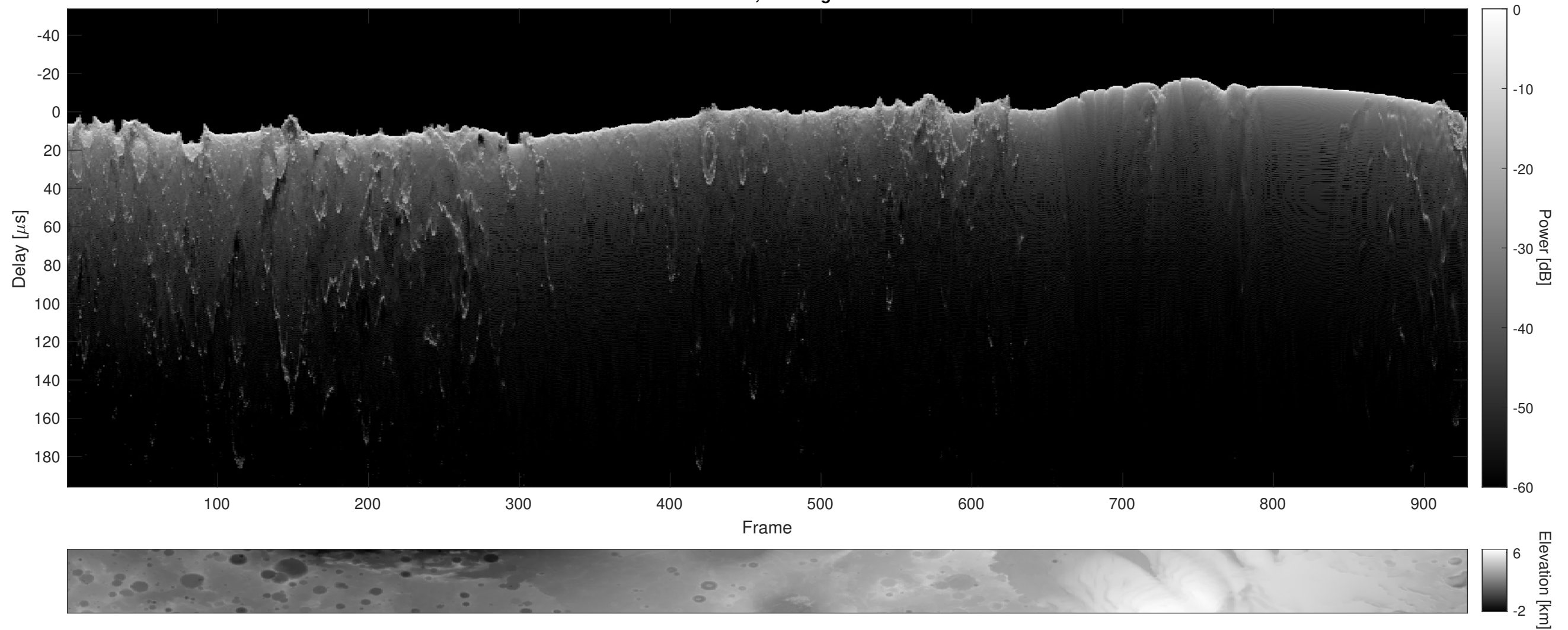
Orbit 6736, Cluttergram
