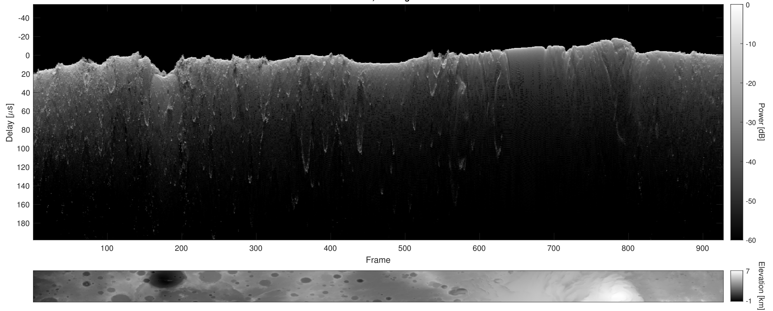
Orbit 6738, Cluttergram
