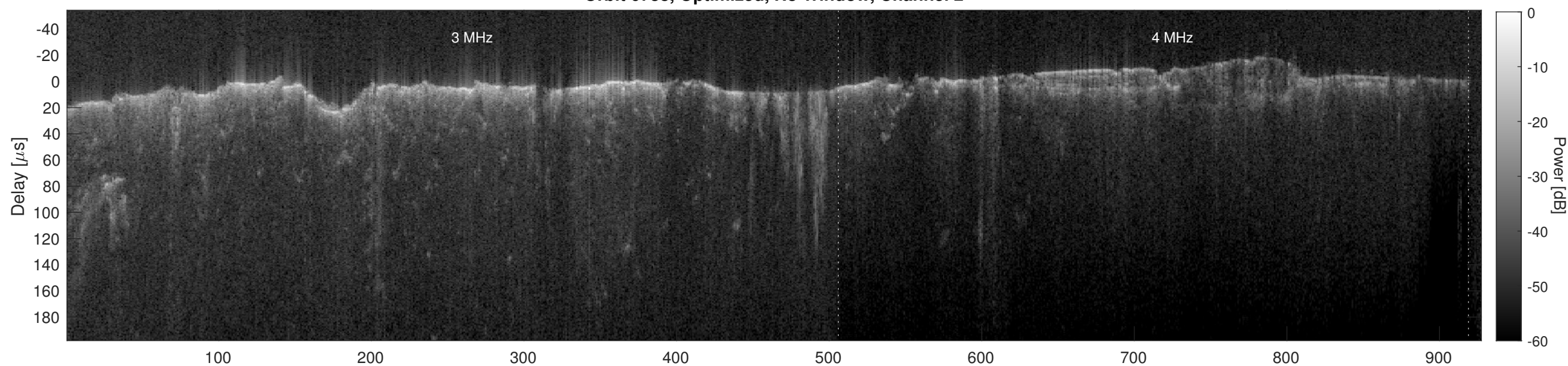
Orbit 6738, Cluttergram
