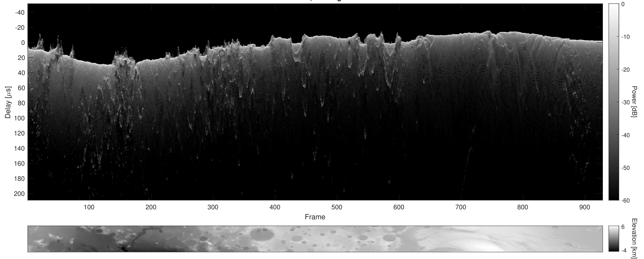
Orbit 6739, Cluttergram
