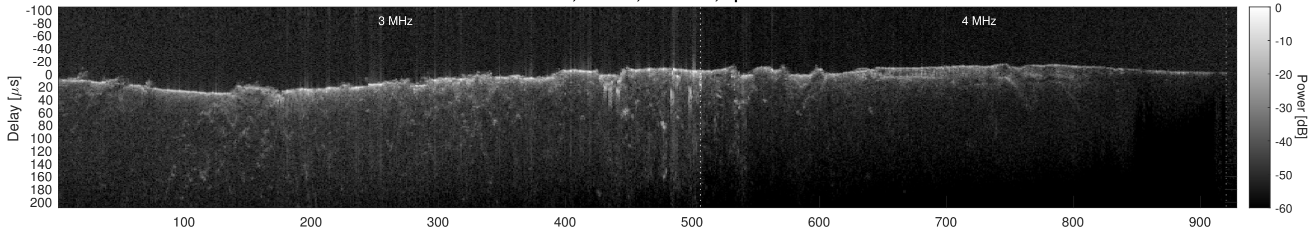
Orbit 6739, Cluttergram
