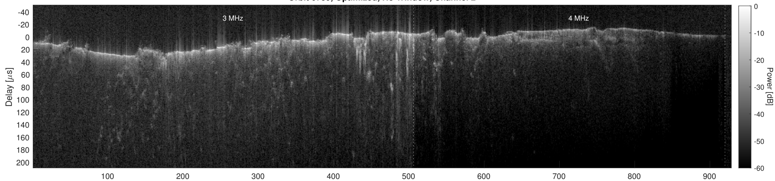
Orbit 6739, Cluttergram
