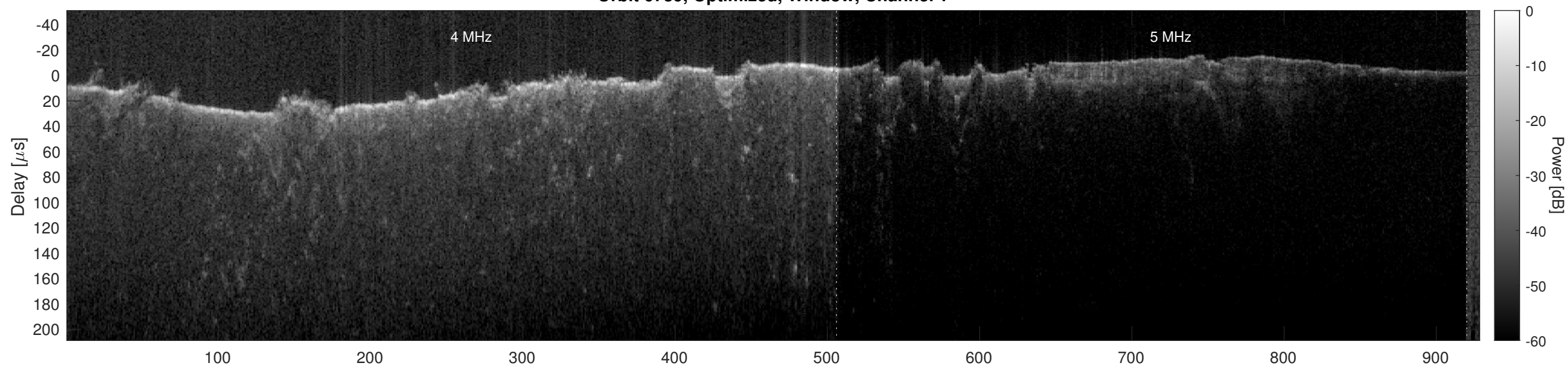
Orbit 6739, Optimized, Window, Channel 2
