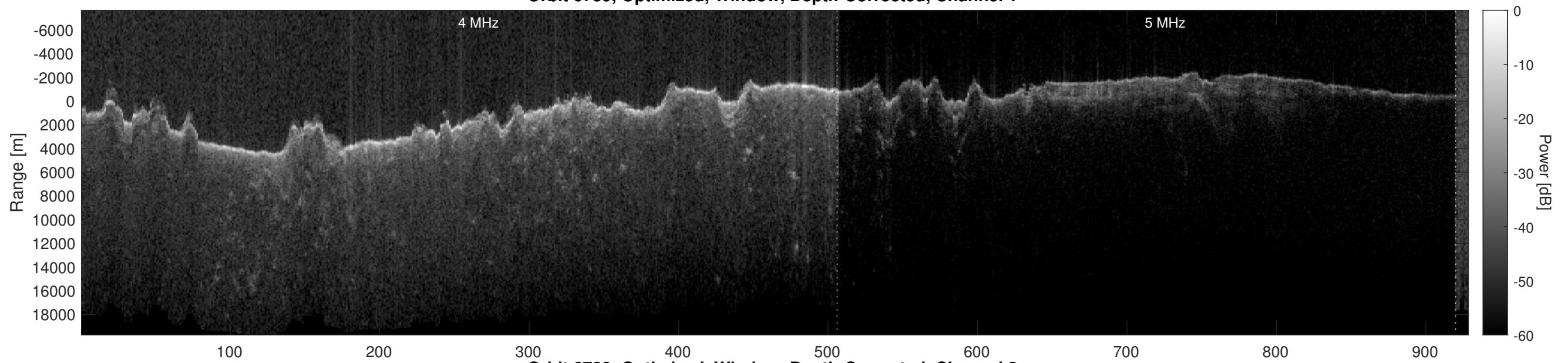
Orbit 6739, Optimized, Window, Depth-Corrected, Channel 2
