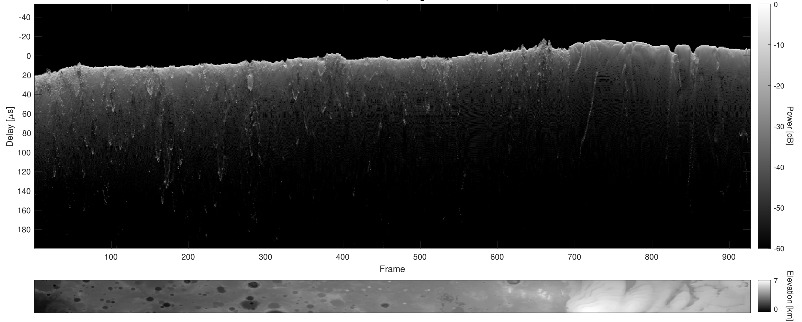
Orbit 6740, Cluttergram
