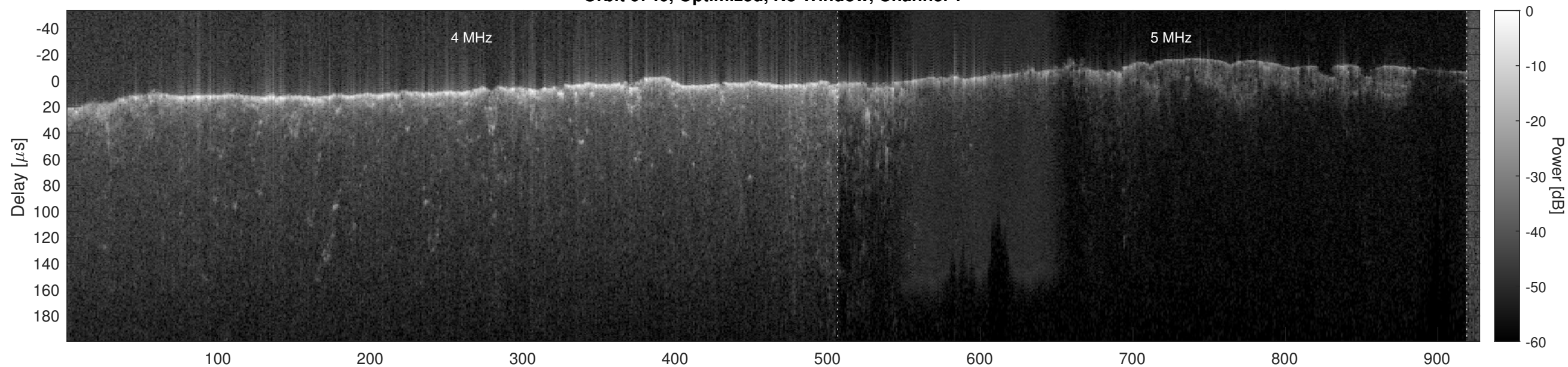
Orbit 6740, Optimized, No Window, Channel 2
