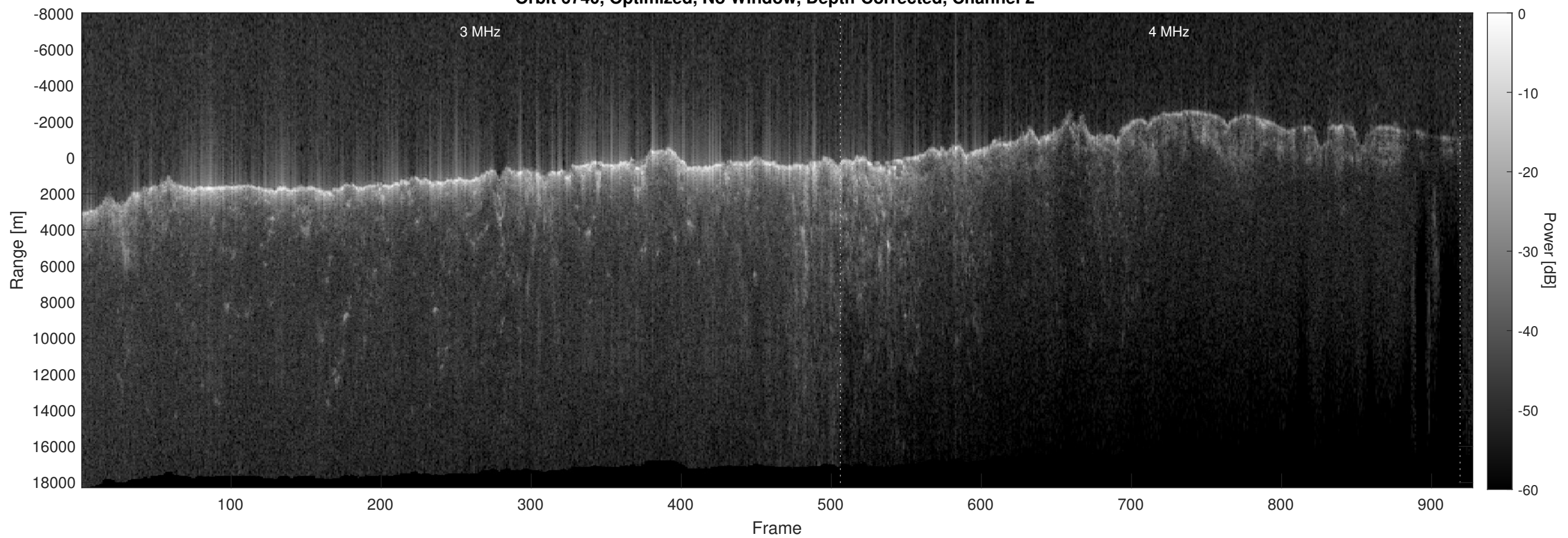
Orbit 6740, Optimized, No Window, Depth-Corrected, Channel 2
