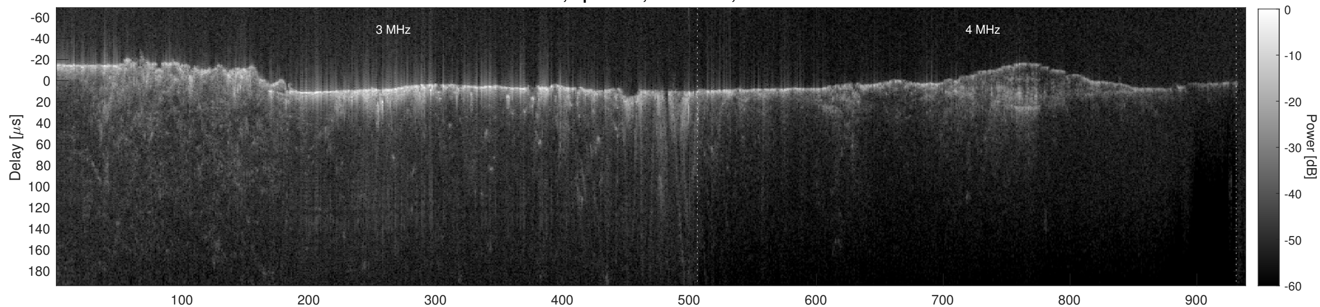
Orbit 6741, Cluttergram
