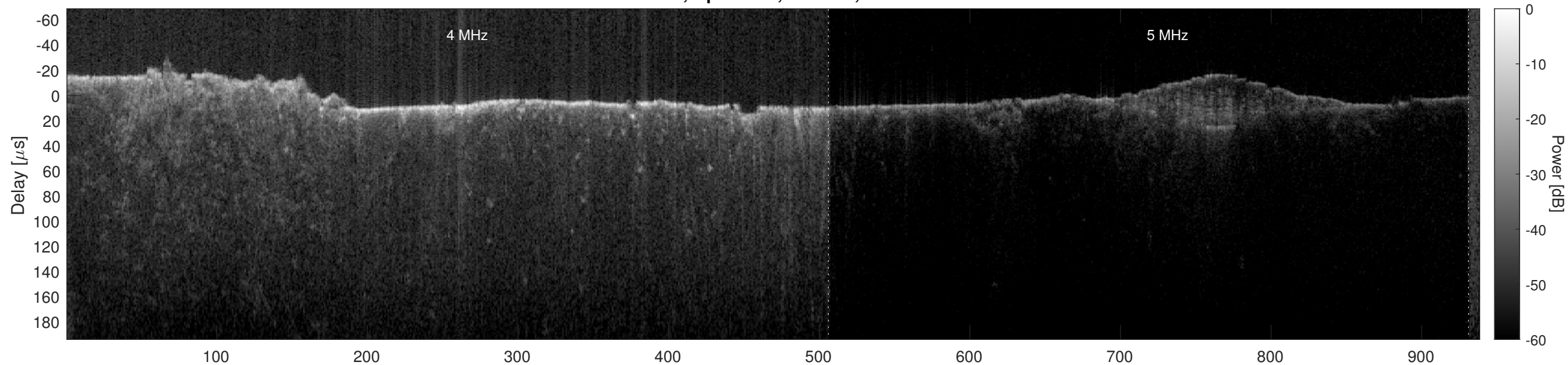
Orbit 6741, Optimized, Window, Channel 2
