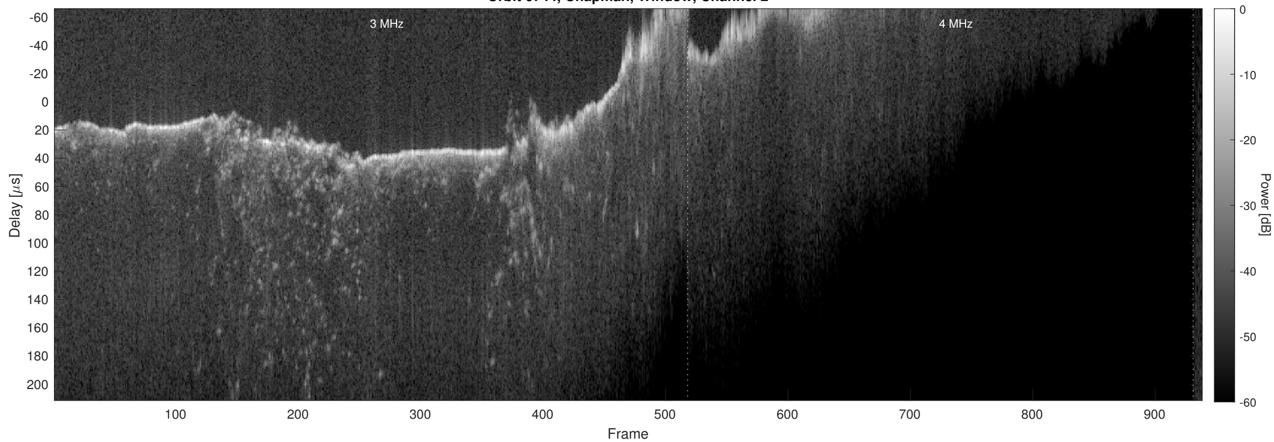
Orbit 6744, Chapman, Window, Channel 2
