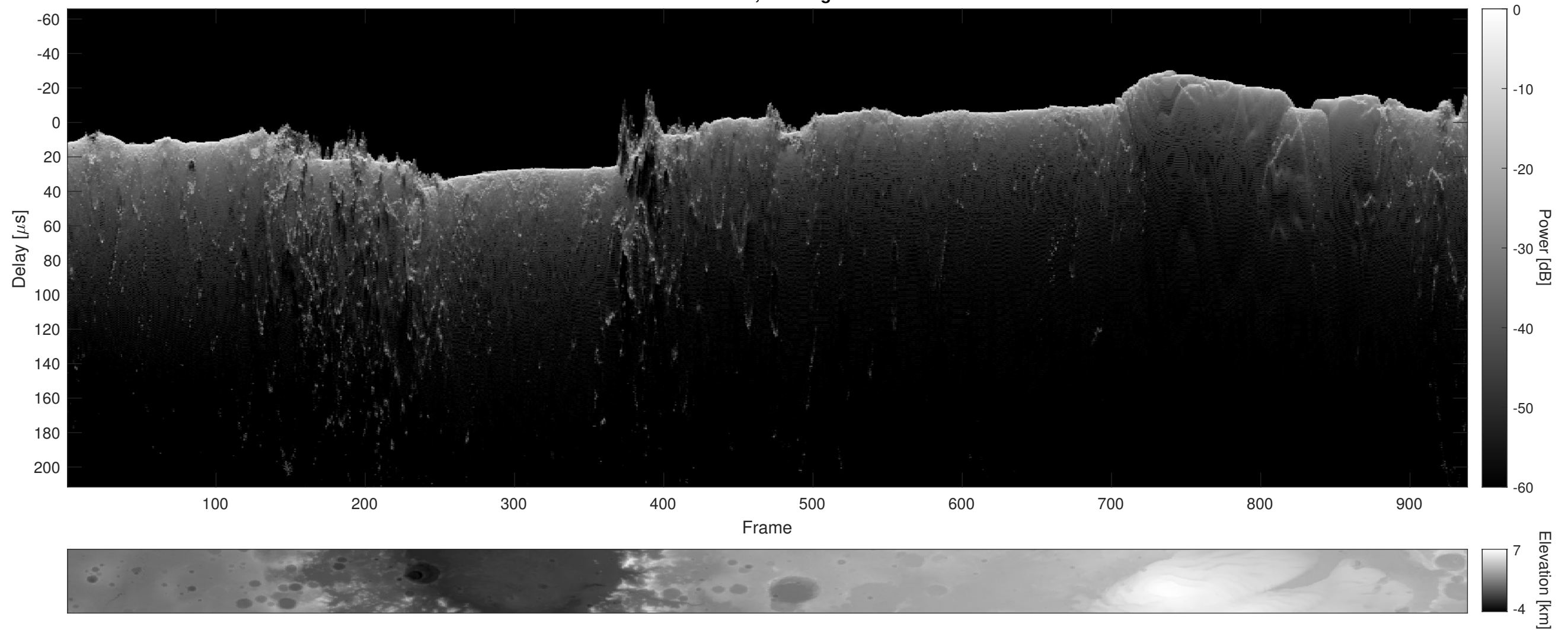
Orbit 6744, Cluttergram
