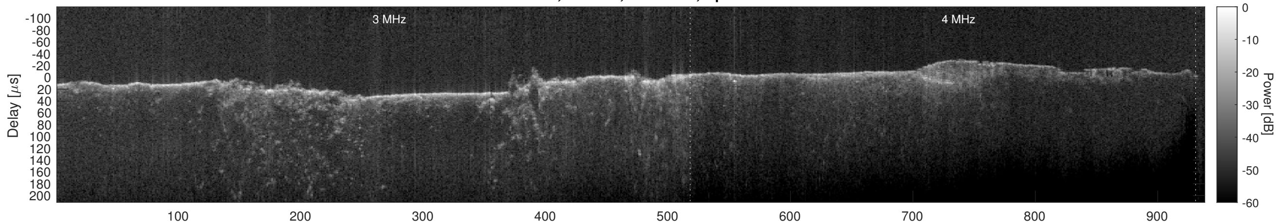
Orbit 6744, Cluttergram
