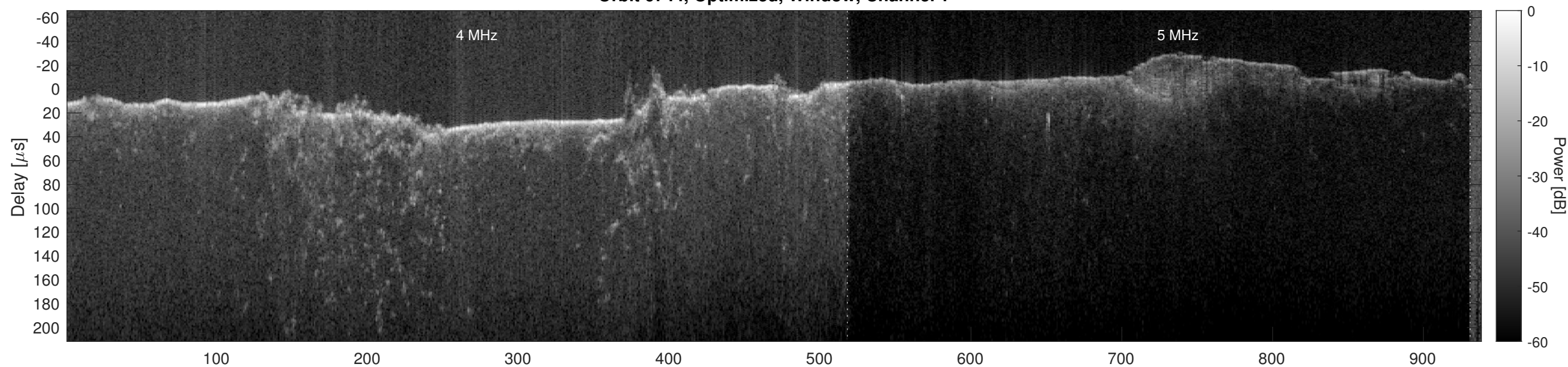
Orbit 6744, Optimized, Window, Channel 2
