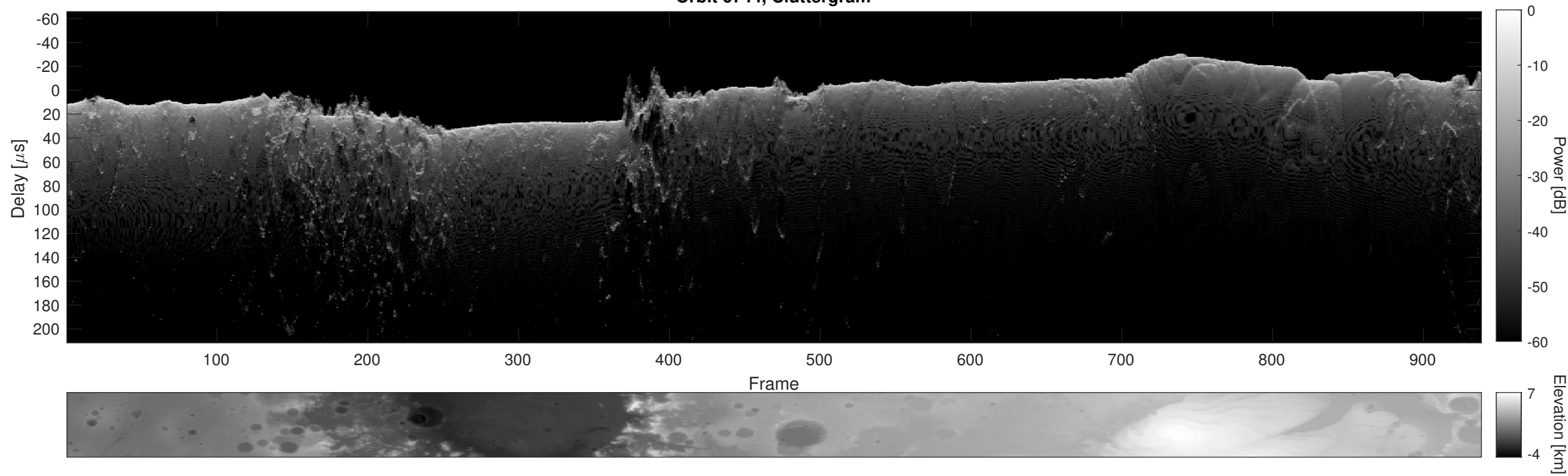
Orbit 6744, Cluttergram
