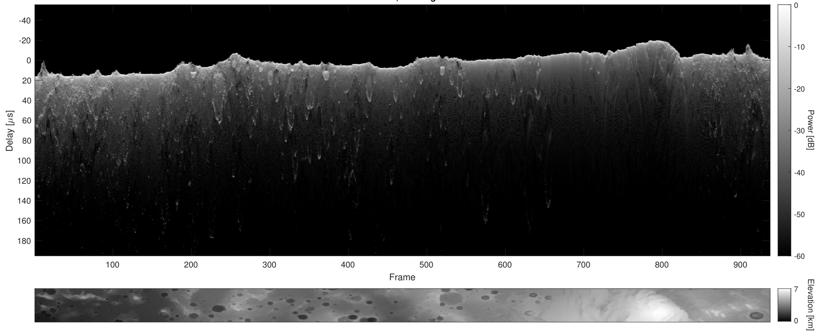
Orbit 6745, Cluttergram
