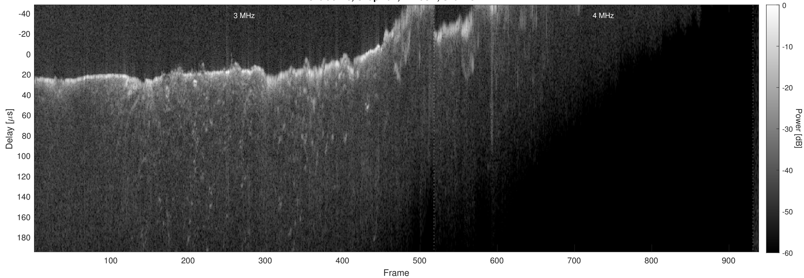
Orbit 6746, Chapman, Window, Channel 2
