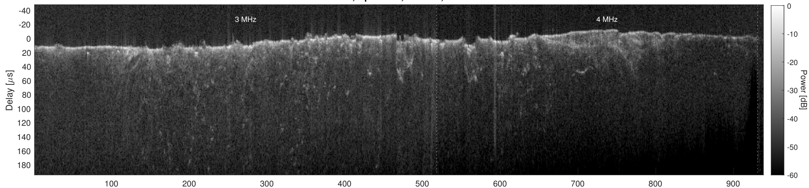
Orbit 6746, Cluttergram
