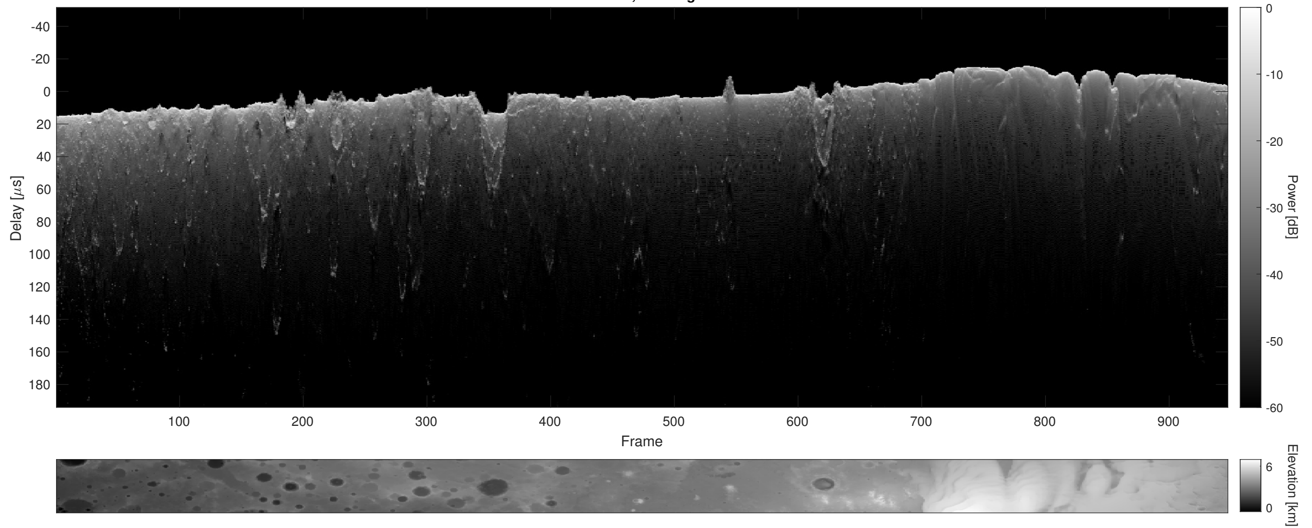
Orbit 6747, Cluttergram
