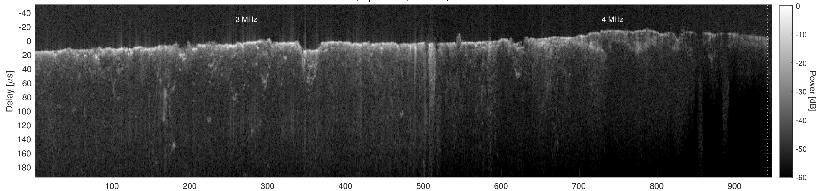
Orbit 6747, Cluttergram
