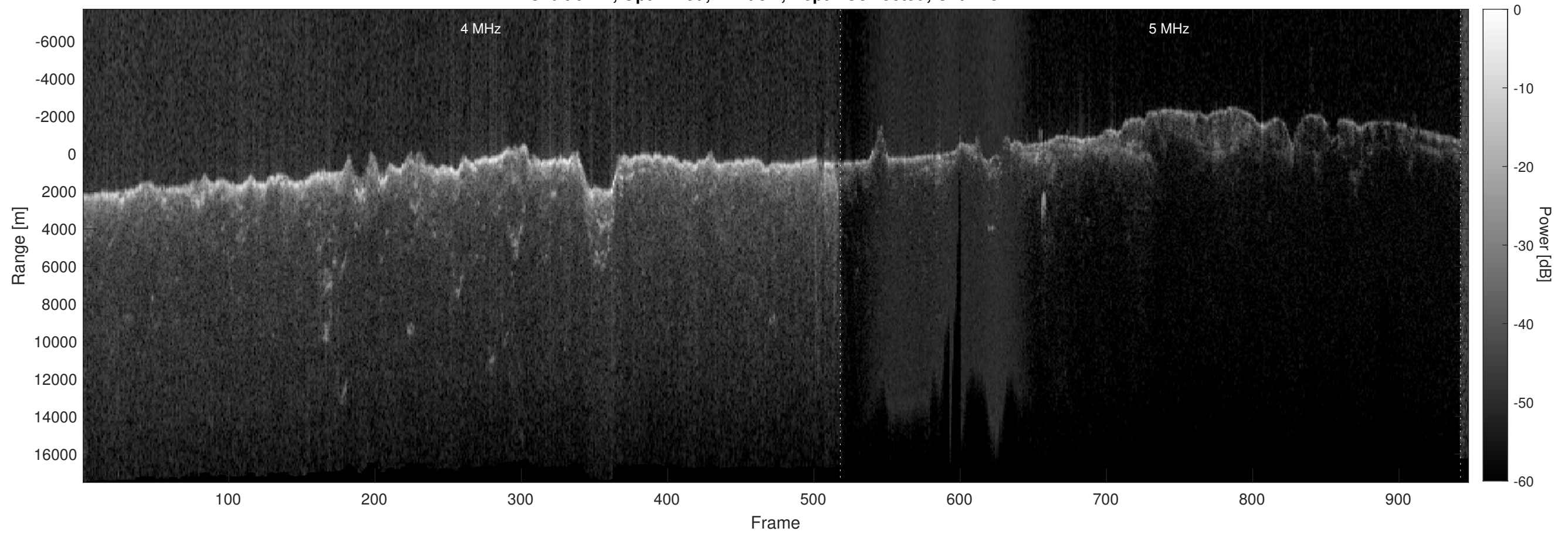
Orbit 6747, Optimized, Window, Depth-Corrected, Channel 2
