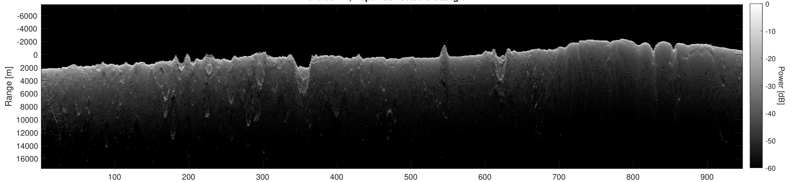
Orbit 6747, Depth-Corrected Cluttergram
