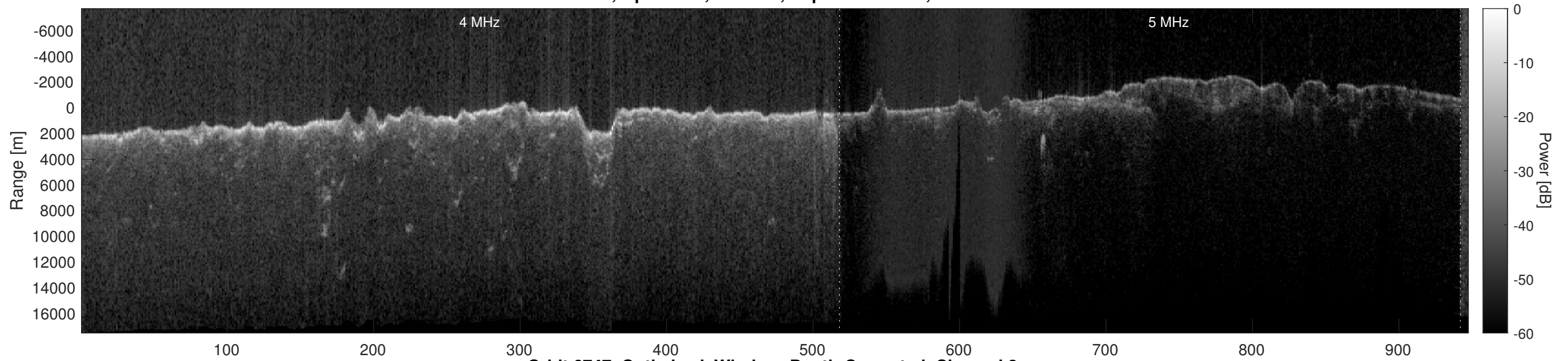
Orbit 6747, Optimized, Window, Depth-Corrected, Channel 2
