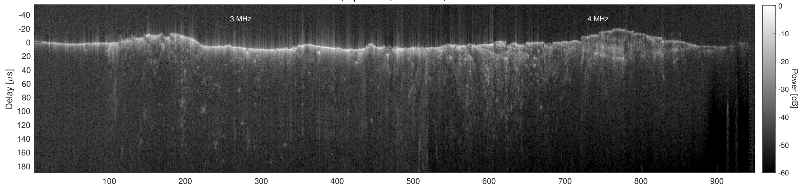
Orbit 6748, Cluttergram
