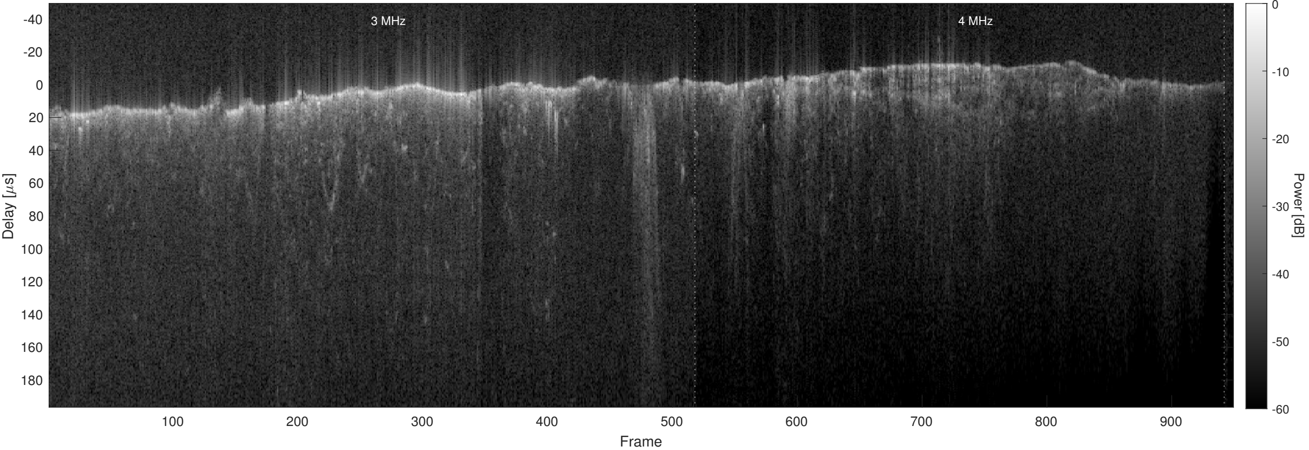
Orbit 6749, Optimized, No Window, Channel 2
