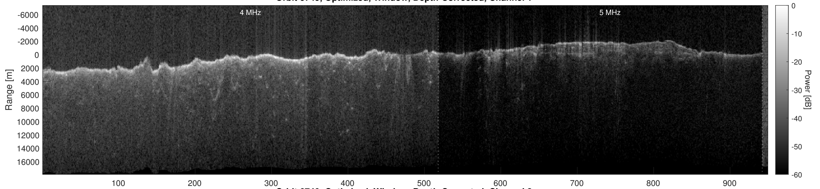
Orbit 6749, Optimized, Window, Depth-Corrected, Channel 2
