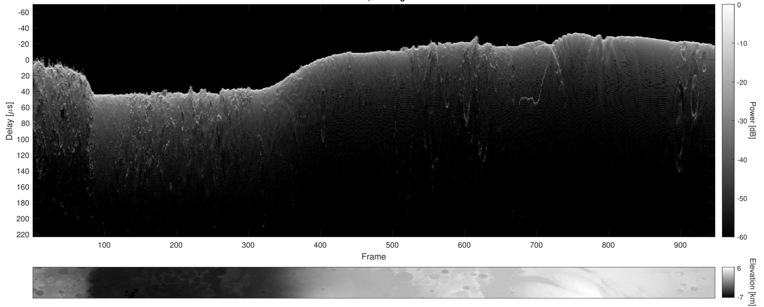
Orbit 6750, Cluttergram
