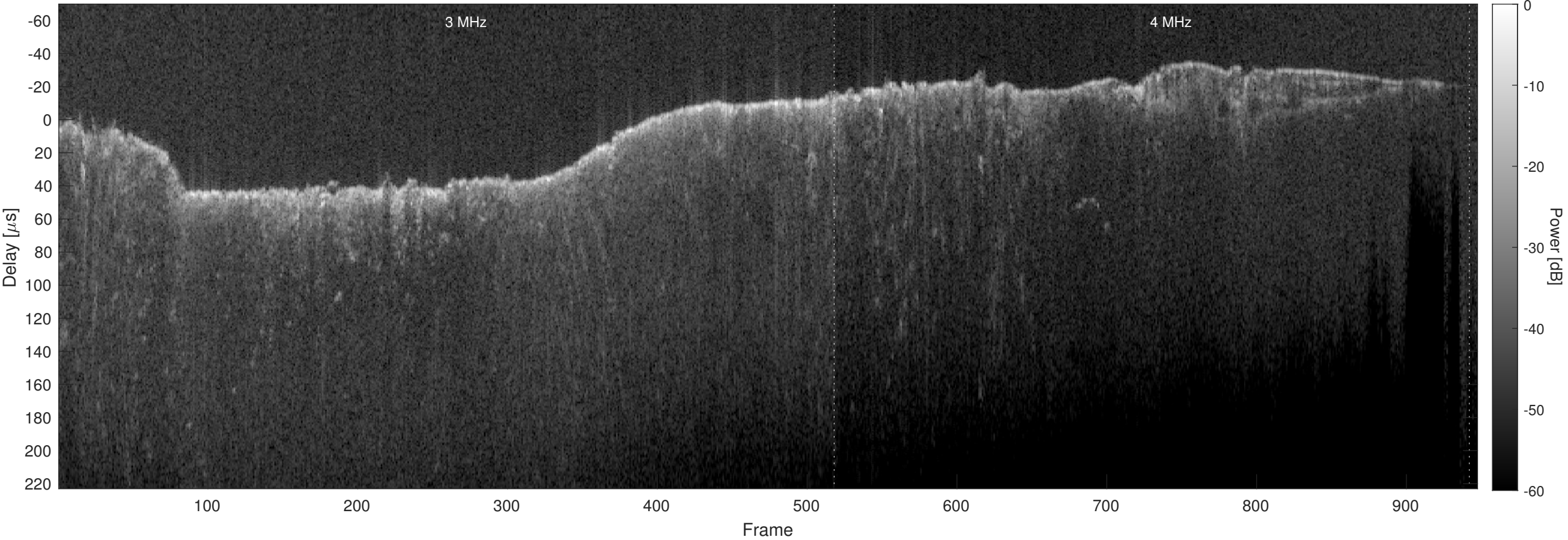
Orbit 6750, Optimized, Window, Channel 2
