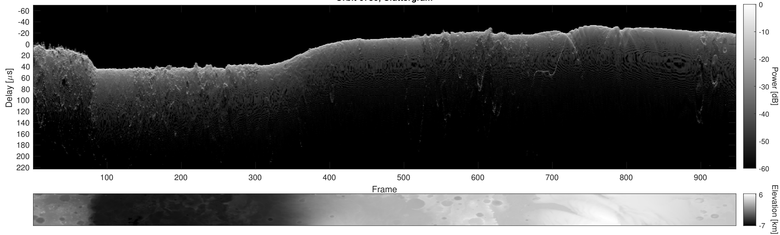
Orbit 6750, Cluttergram
