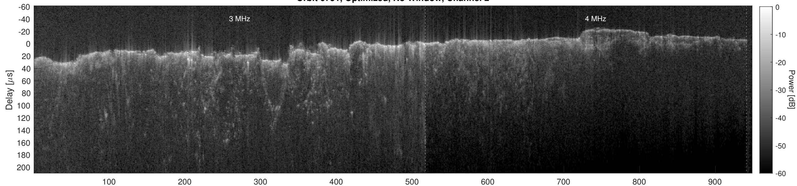
Orbit 6751, Cluttergram
